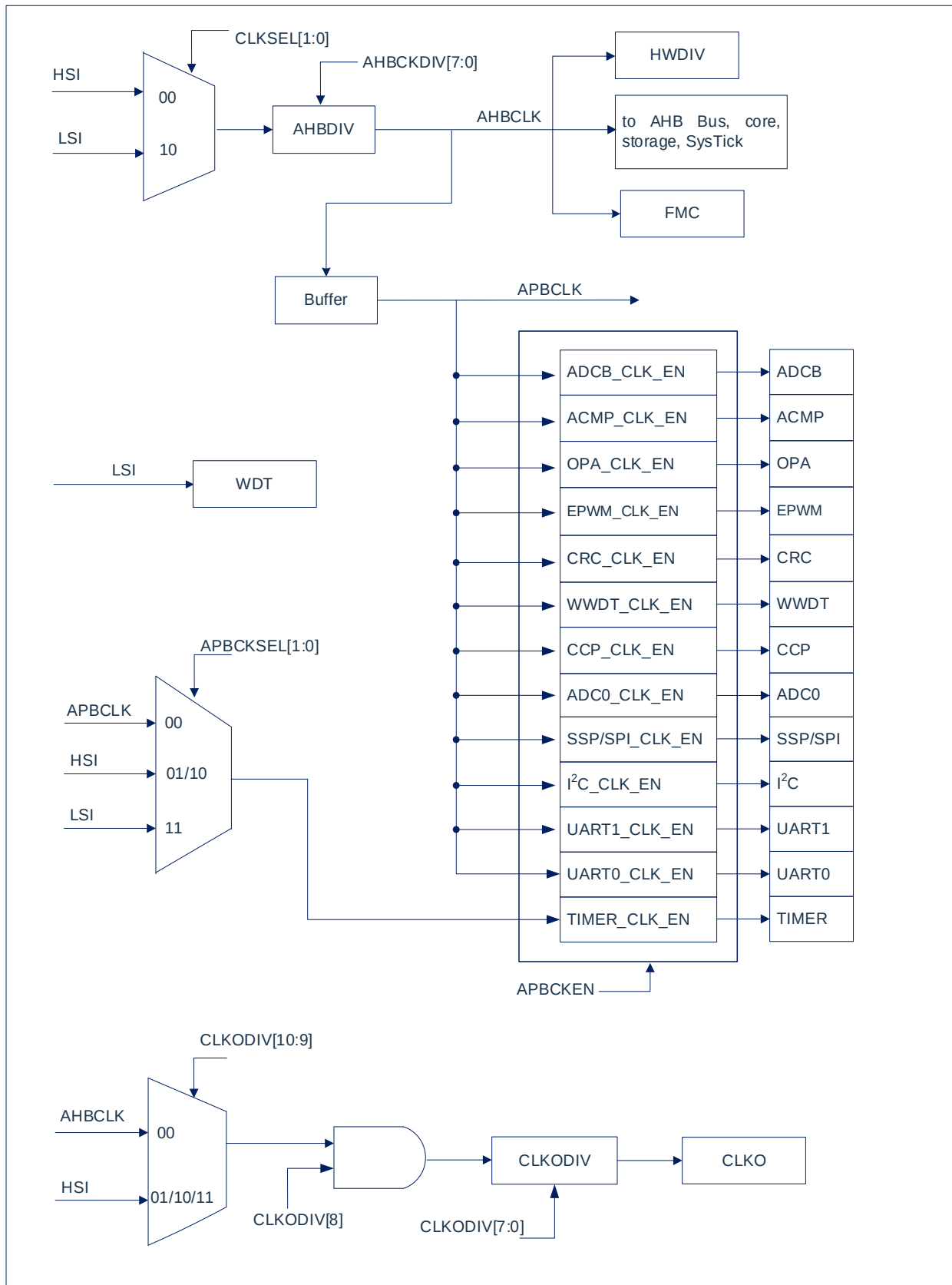
Figure3-2: Clock control block diagram
